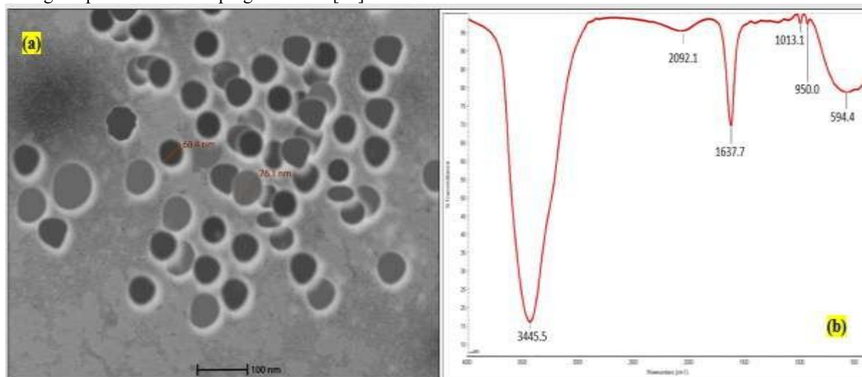
Figure 7. (a) TEM image of TPHE-mediated ZnO NPs, (b) FTIR spectrum of TPHE-mediated ZnO NPs.
